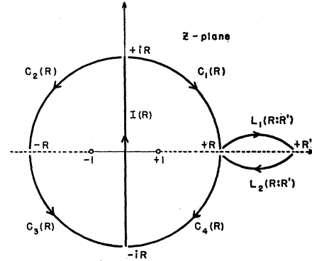
FIG. 3. Special contours used in the discussion of the contour integral representation of the sum over the energy states.
